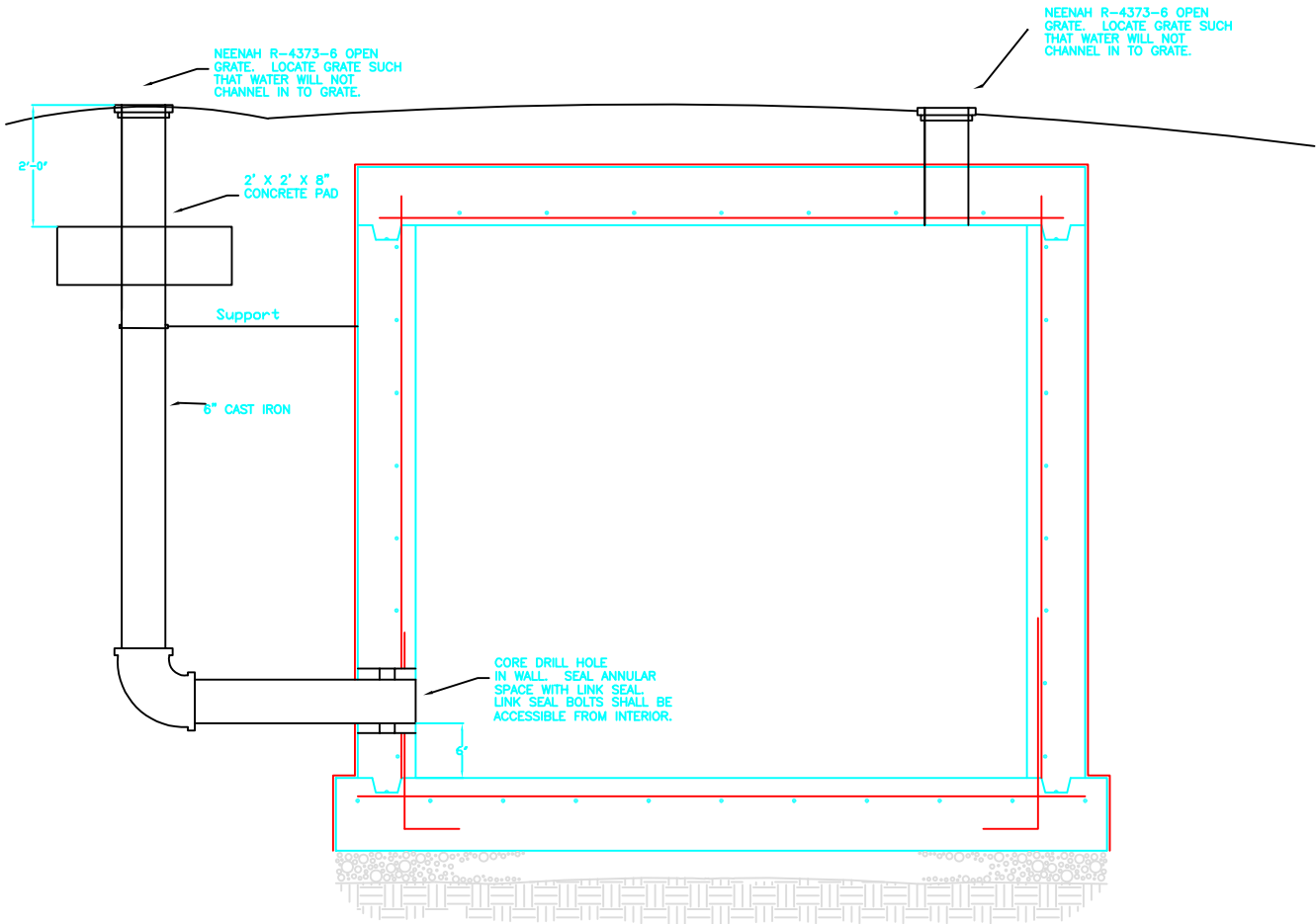
MANHOLE VENT DETAIL
