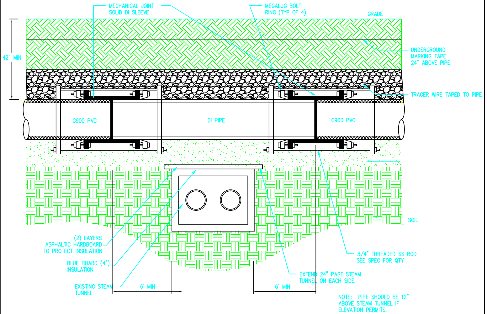
X MX STEAM CHASE/TUNNEL CROSSING DETAIL NO SCALE
