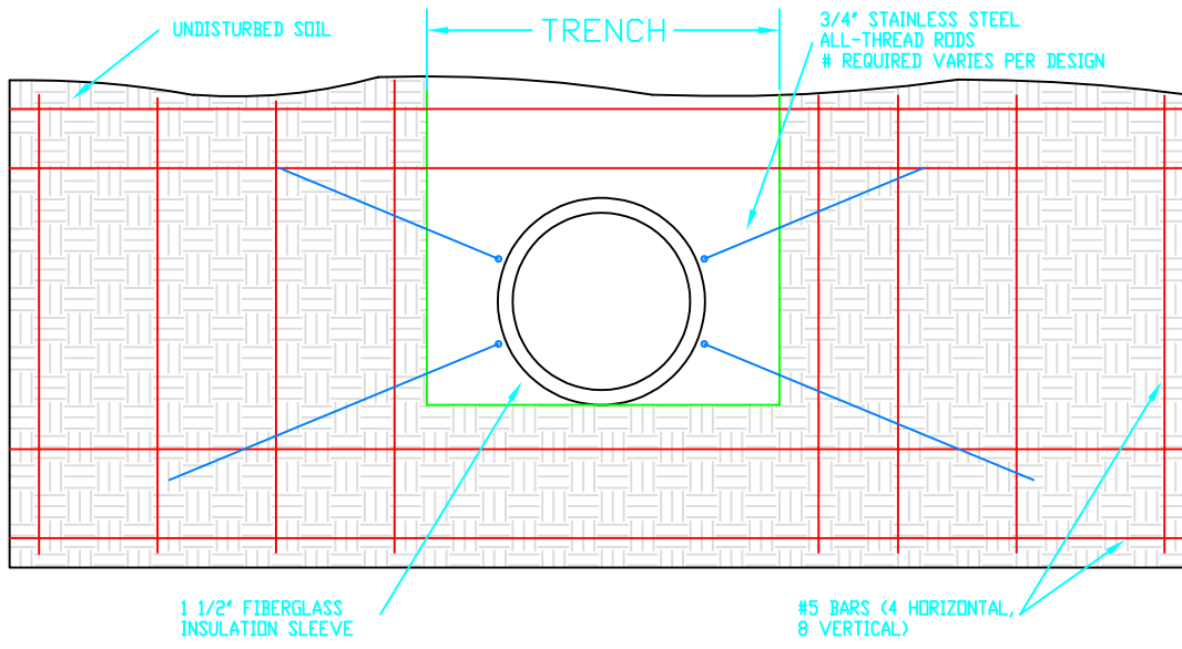
SECTION
