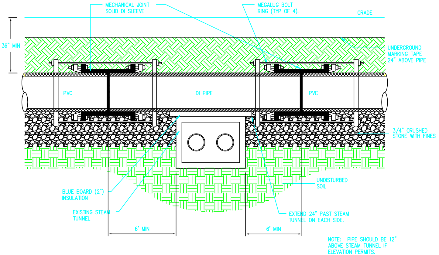
X MX STEAM CHASE CROSSING DETAIL NO SCALE
