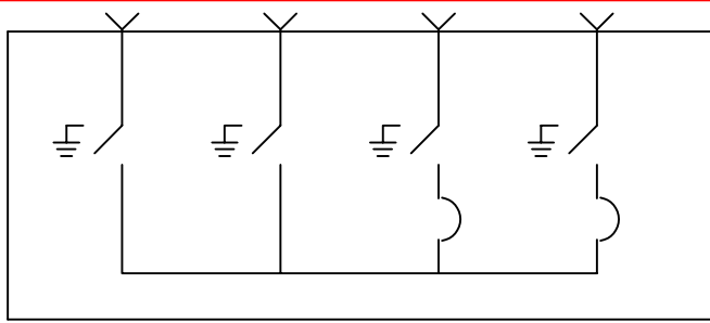
4-WAY (422)
