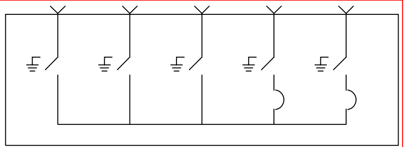
5-WAY (532)
